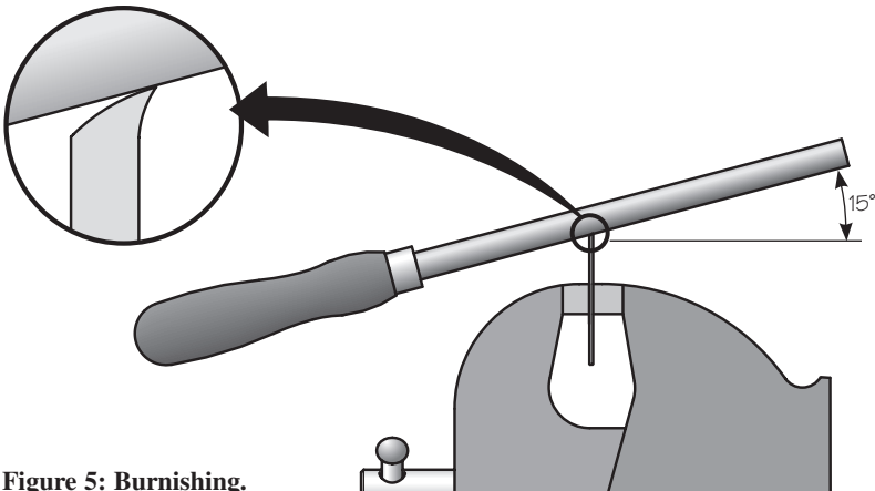
Figure 5: Burnishing.
