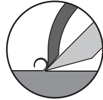
Figure 2b: Bench plane with well-set cap iron.
